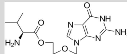
Valacyclovir L-valyl ester of acyclovir
