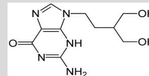
Penciclovir acyclic guanosine analog retains 3' group It is not an obligate chain terminator.
