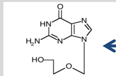
Acyclovir acyclic guanosine analog (lacks 3' -OH)
