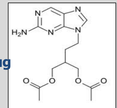
Famciclovir diacetyl ester of 6-deoxypenciclovir
